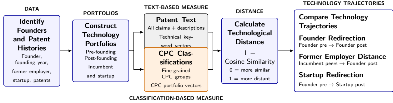
Figure 2: Construction of Technological Distance Measures.
